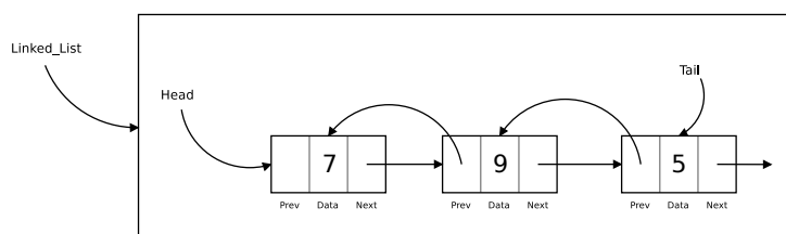
Figure 111: A doubly linked list is an example of redundancy
